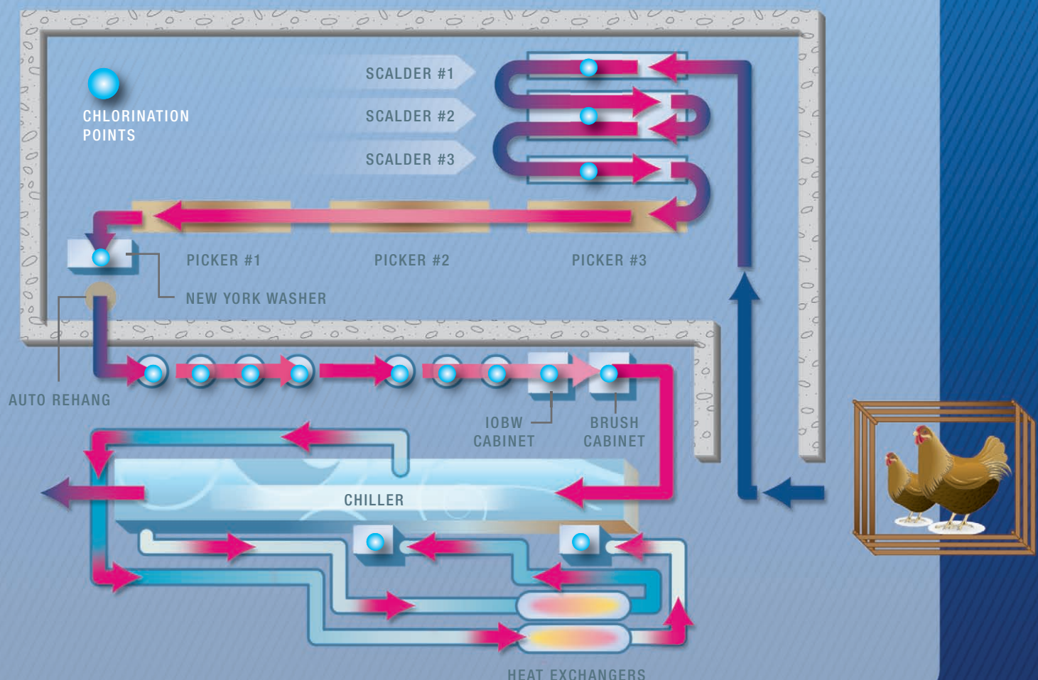
POULTRY PROCESSING DIAGRAM
